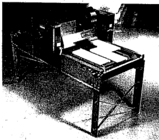
Measures 6 feet in length and is 30 inches wide, except in the flail drive area which is 39 inches wide and 25 inches high. Weight: 350 lbs. Crated weight: approx. 420 lbs.
